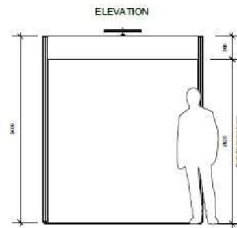
Fabric Booth 2x2 Inline
